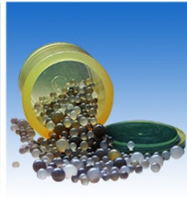
PU planetary mill jar with agate balls
